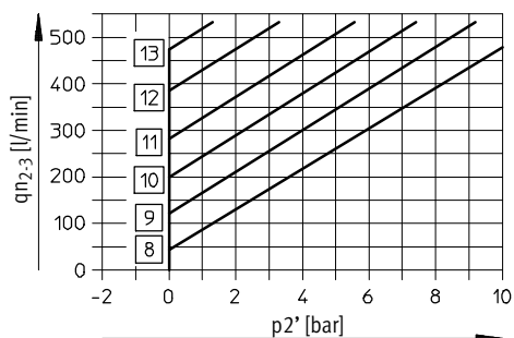
Standard flow rate q_{n2-3} of the secondary exhaust as a factor of the excess output pressure p_2'
