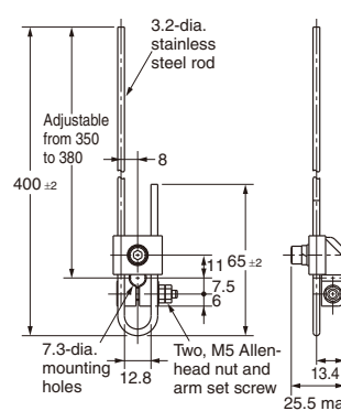
WL-3A106 Double Nut
